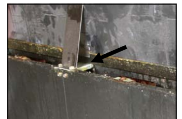
Figures 3,4: Attach flue cap extension with removed screws and provided drill-point screws at positions indicated by arrows. A flange (see photo, right) on the flue cap extension grips the existing flue cap behind the middle brace.
